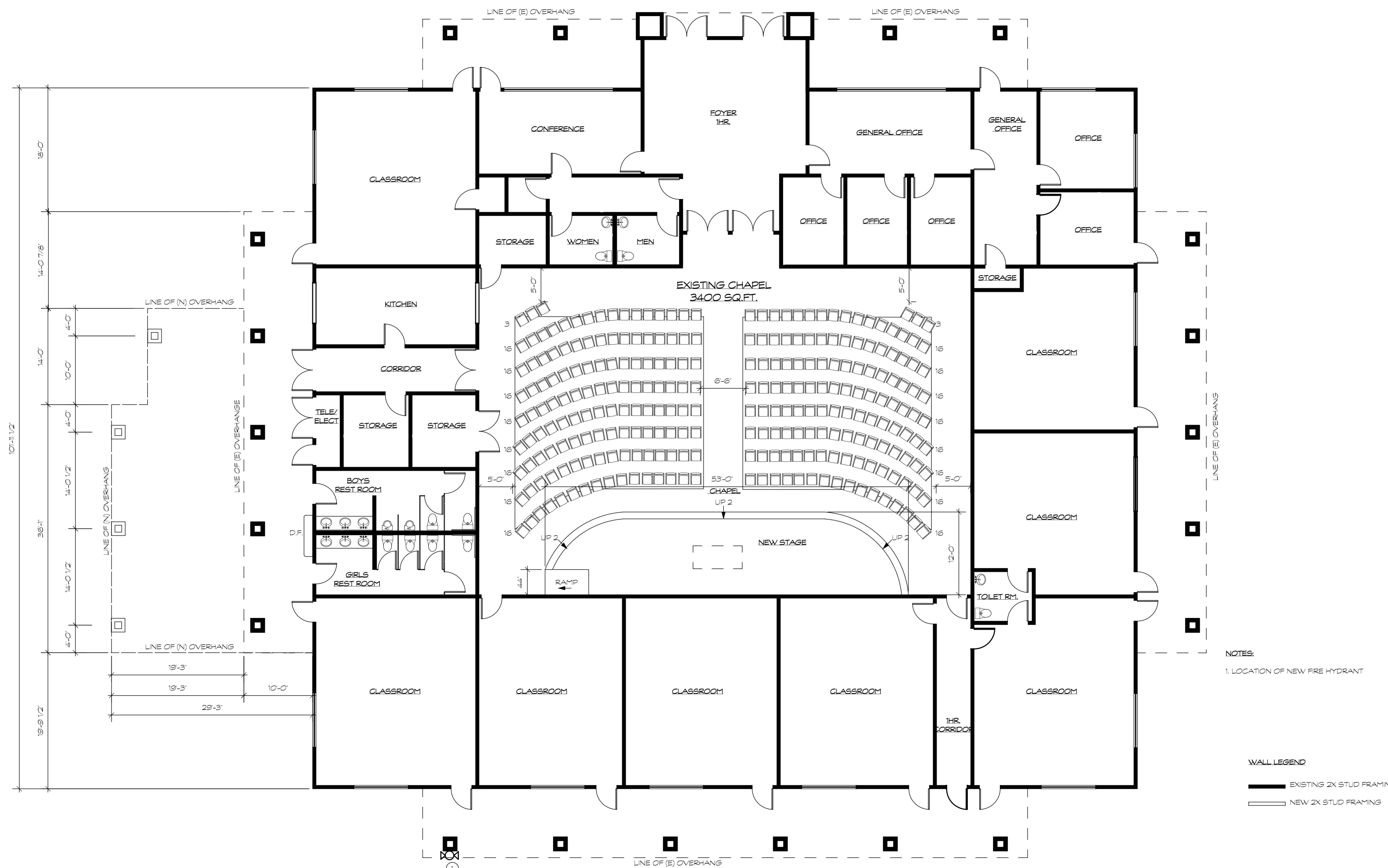
1 PROPOSED CHAPEL/CLASSROOM RENOVATION Scale: 1/8" = 1'-0"
